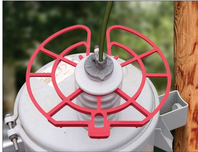
Model W-1525R ZAPSHIELD Installed on a Distribution Transformer.
