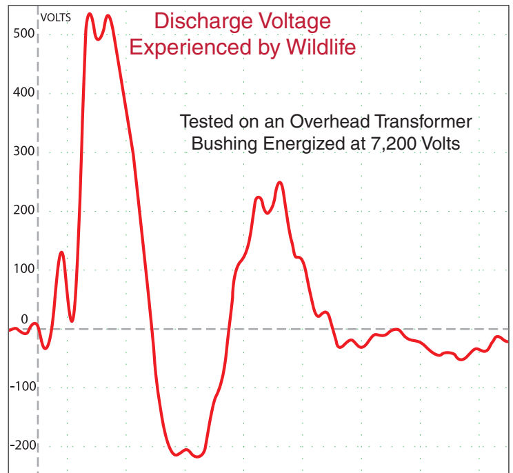
Voltage Discharge Curve for a ZAPSHIELD Installed on a 7,200 V Distribution Transformer Bushing.
